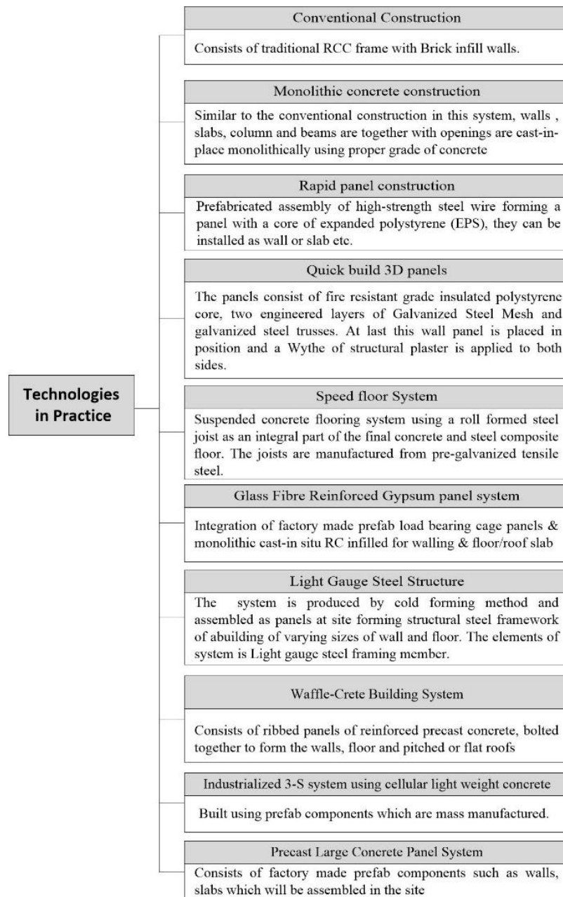
Figure 1. Low-cost housing technologies used in practice (adapted from BMTPC, 2015)
