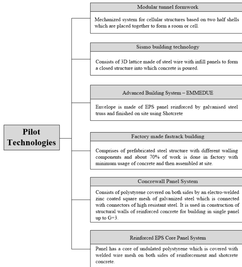
Figure 2: Pilot technologies for Low-cost Housing (adapted from BMTPC, 2015)
