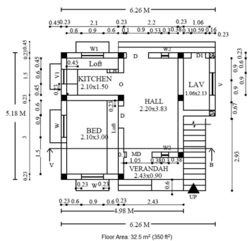
Figure 4. Floor plan of a typical EWS type dwelling unit (Devi and Palaniappan, 2018)
