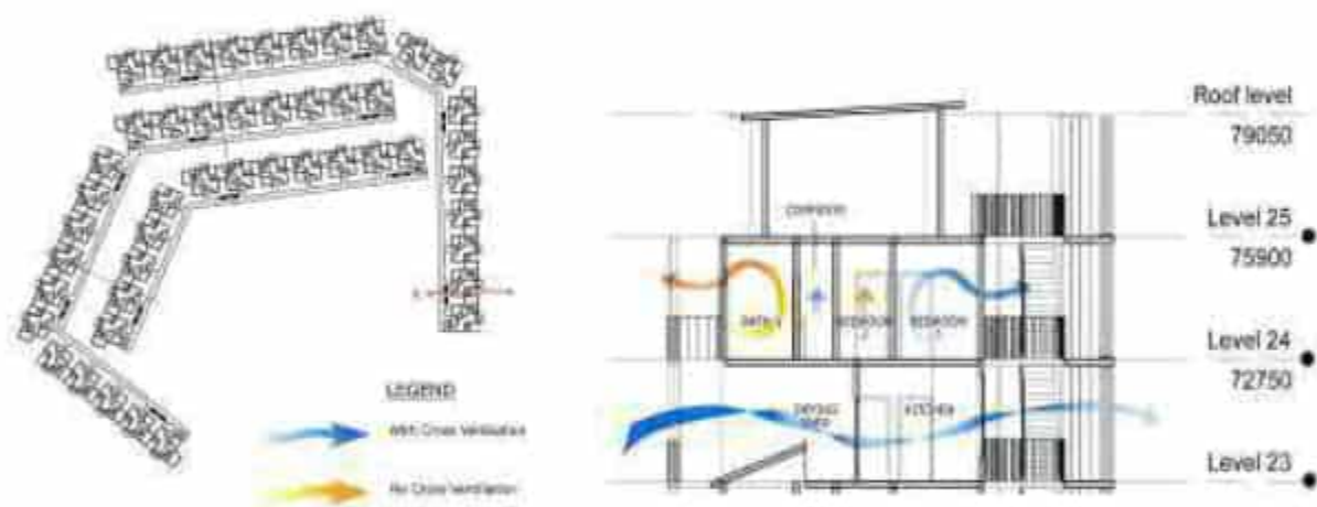
Figure 2.30 Natural Ventilation Analysis for Section 1
