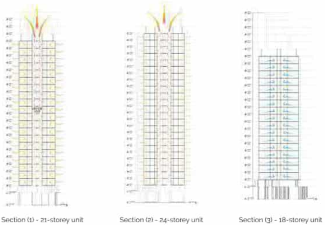
Figure 2.20 Natural Ventilation Analysis for Building Section at Different Height
