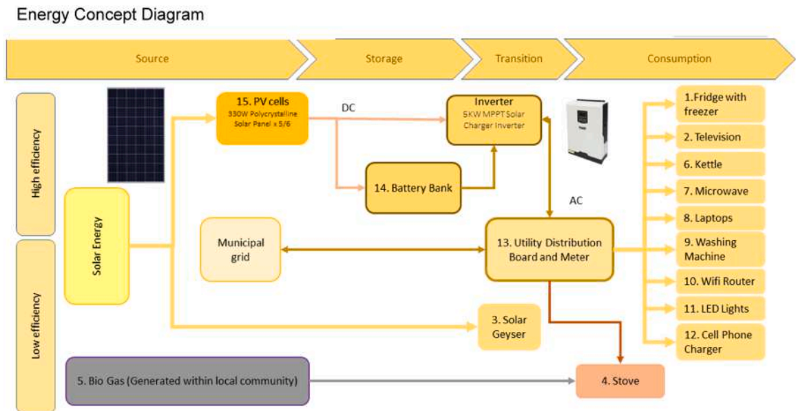
Fig. 7. Energy and water usage design concepts. Source Phiri and Bosa. 2021.
