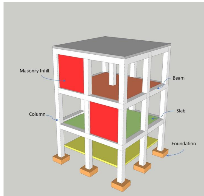
Diagram 1: Conventional construction
