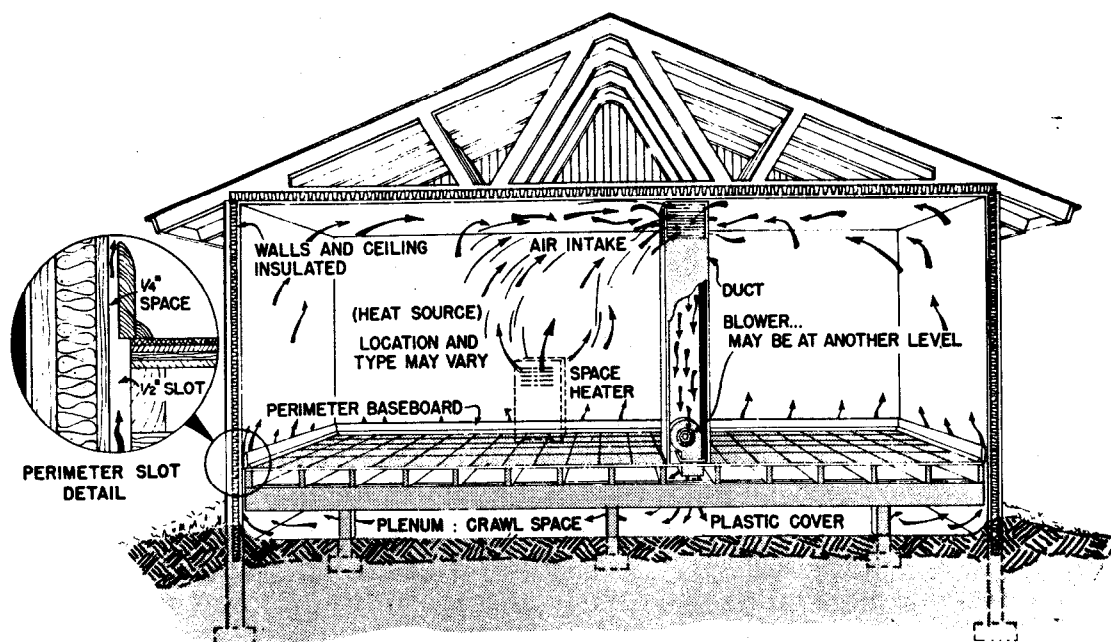
AIR DIFFUSION SYSTEM USING UNDER-FLOOR PLENUM WITH PERIMETER SLOT
